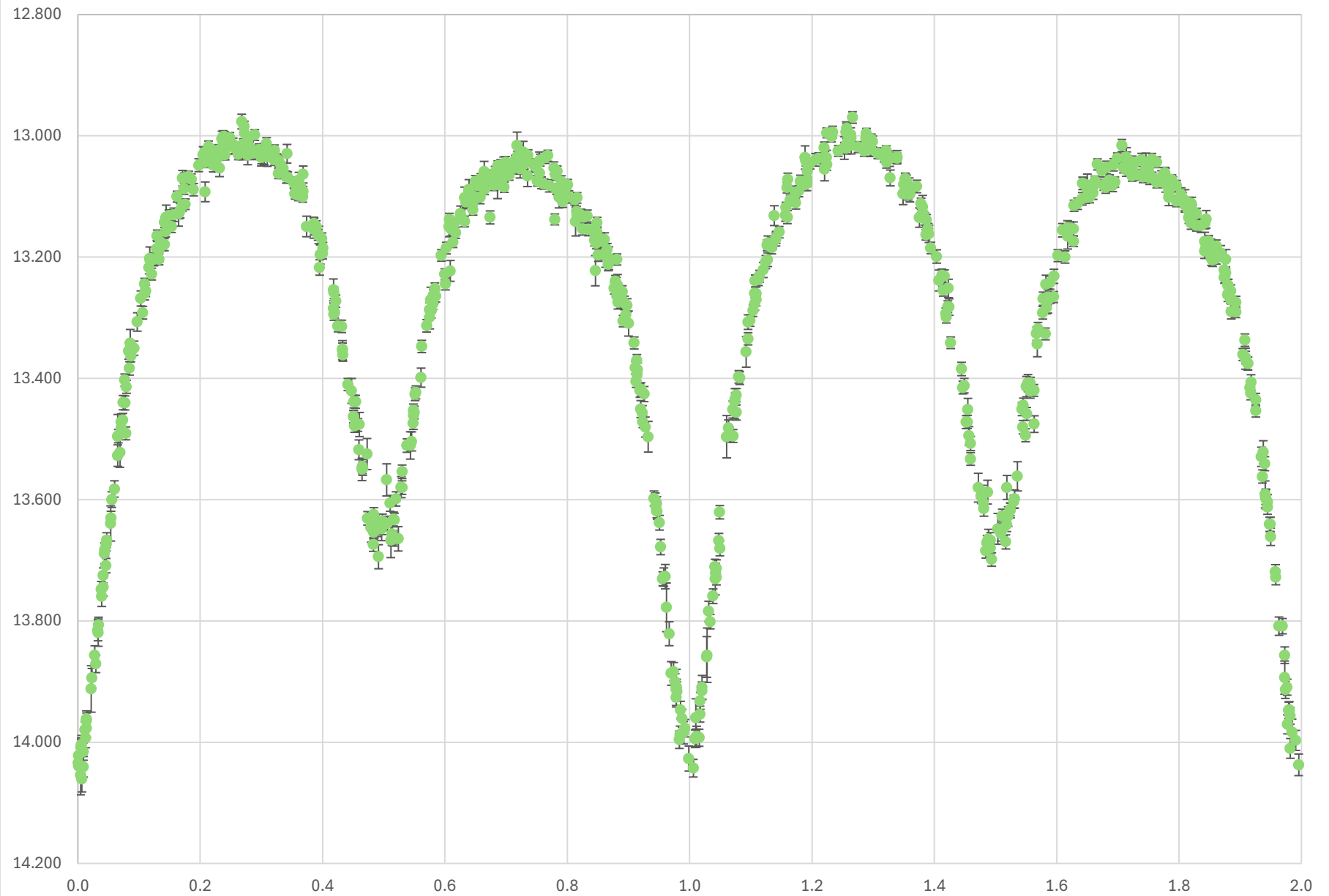
ASAS J221652+2229.6 V-Filter Source_AMag_T1
